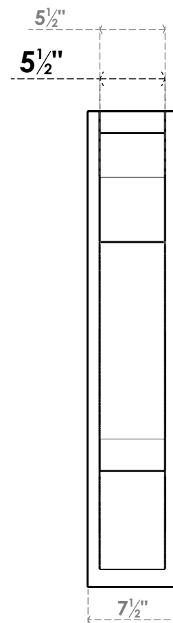
FRONT PROFILE
